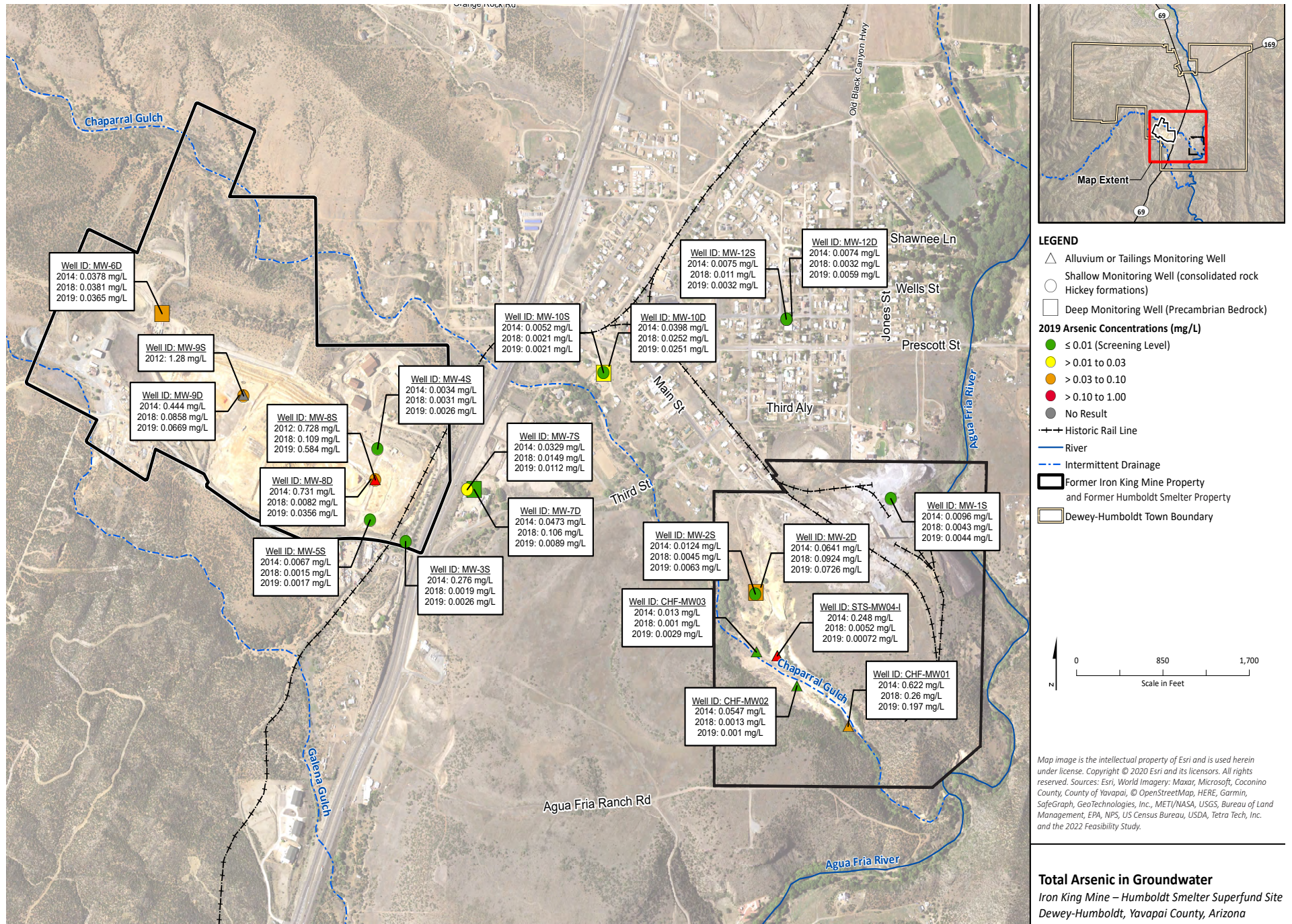
Figure 7. Total Arsenic In Groundwater
